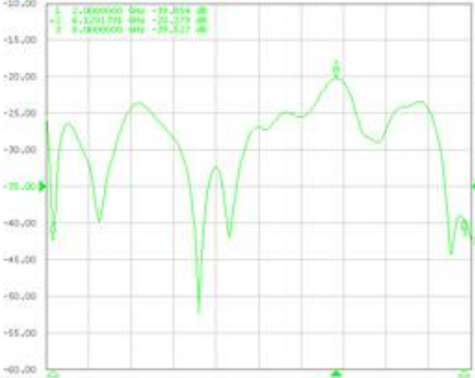
Tr3 S22 Log Mag 5.000dB/ Ref -25.00dB [F2]
