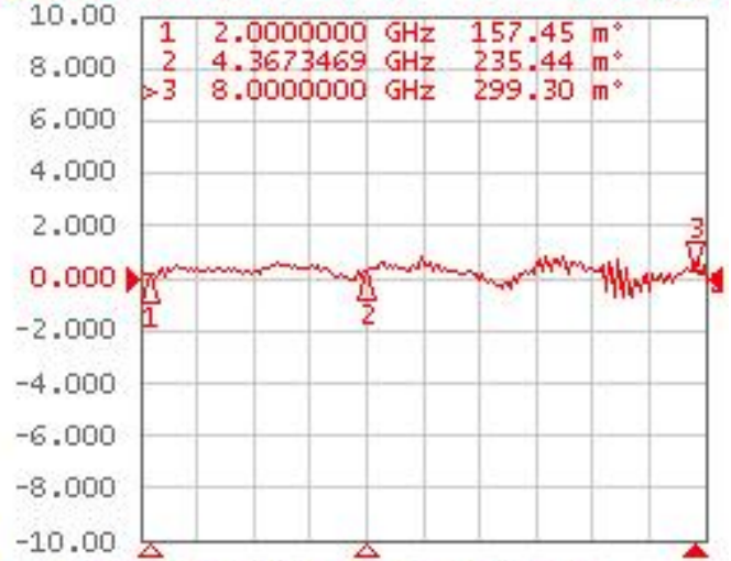
Tr4 S22 SWR 100.0m/ Ref 1.000 [F2]
